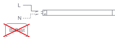
Diagram 3 – Single tube wiring
